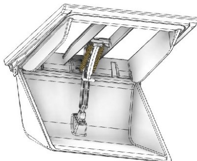
2. Fully open door so that closer assembly can fit through back side of inlet frame
